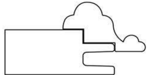
End view of DM-820 molding on Grandview door.
