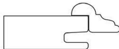
End view of DM-890 moulding on Brookfield door.
