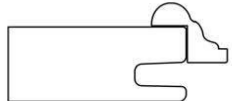
End view of DM-870 molding on Hartford door.
