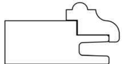
End view of DM-800 molding on Harvard door.
